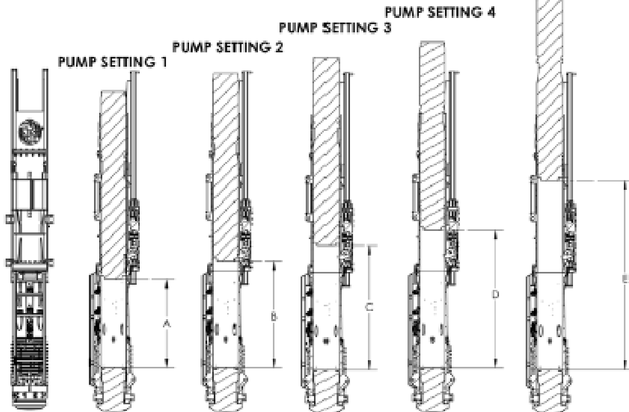
STROKE TO CATCH RING
