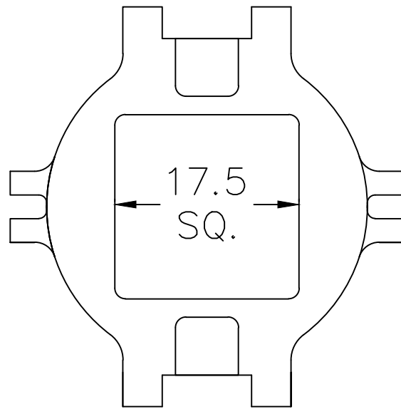
32" DRIVE CAP BASE Wt. = 2750 lb.
