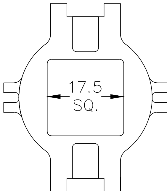
37" DRIVE CAP BASE Wt. = 2976 lb.
