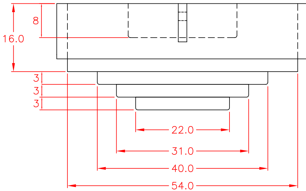
54" STEP-TAPERED PIPE HELMET Wt. = 13,050 lb.
